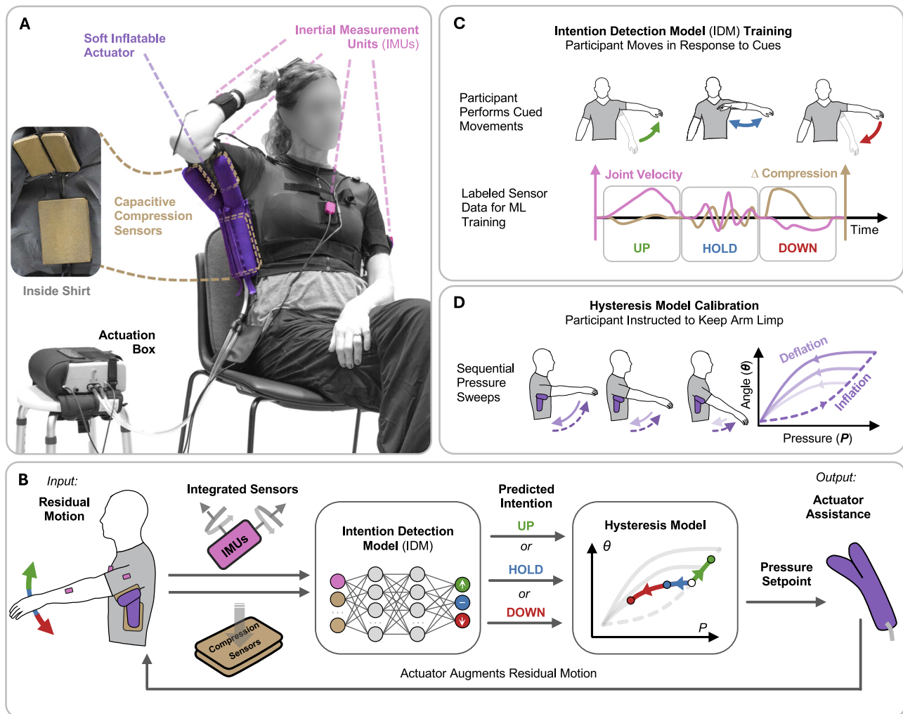
Fig. 1 | Overview of the soft wearable robot and high-level control strategy.
